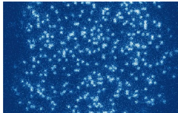
Snapshot of the individual atoms of strontium in the optical lattice
