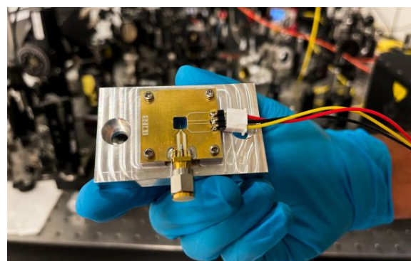
Evaluation kit featuring the fabricated printed circuit board with the integrated graphene sub-terahertz receiver, mounted on a metal support. Credit: ICFO.
