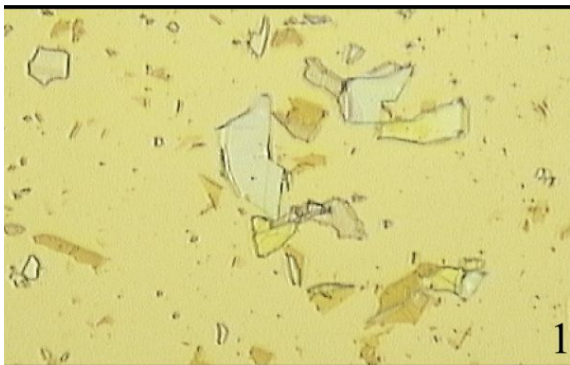
Microscope image of exfoliated hBN flakes on a gold substrate. Source: npj Nanophotonics.
