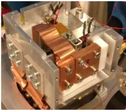
The home-built nanositioner used to move the fiber in three dimensions over the surface of the mirror. ©ICFO/E. Beattie
