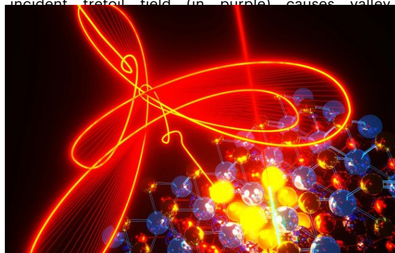
Illustration showing the valleytronics effect. Image credit: ICFO / Ella Maru Studio
