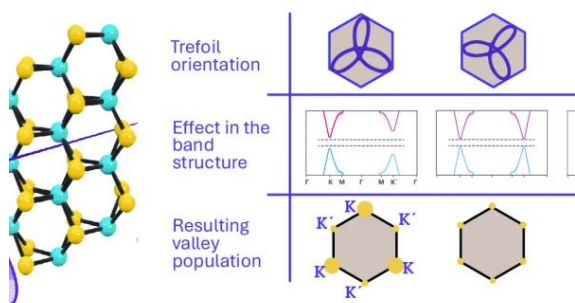
Schematic of the valley polarization effect, where the incident trefoil field (in purple) causes valley
