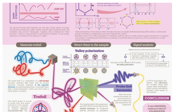
Infographic of Valley Polarization
