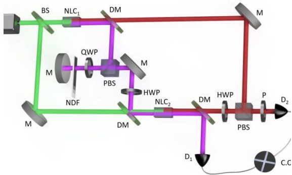
Sketch of the experimental setup.
