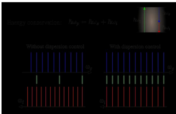
Energy diagram of the process and the cavity modes without (left) and with (right) dispersion compensation. Source: Physical Review Research.
